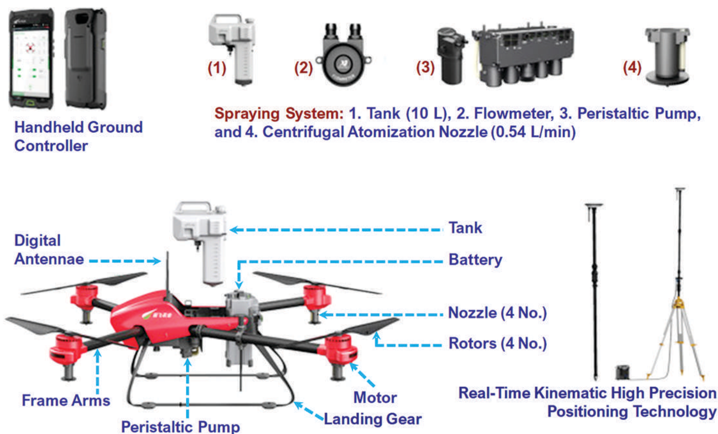
Fig. 1. A spraying UAV (quadcopter) with basic components
